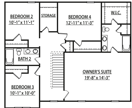
SECOND FLOOR PLAN W/ 2 CAR GARAGE
