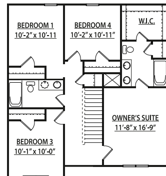
SECOND FLOOR PLAN W/ 1 CAR GARAGE
